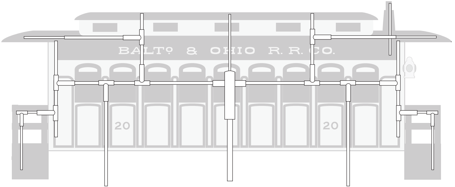
Completed Internal Strut Assembly. Make sure all parts connect as shown.
